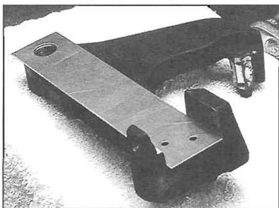
This shot shows Arlen's template in place. The tabs on either side need to be cut off with a hacksaw, then the holes must be drilled and tapped.
