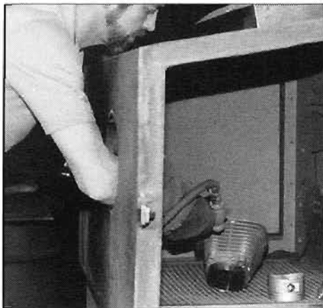
Sand blasting parts is necessary to remove or dislodge baked-on sludge and oil. Afterwards, parts need to be degreased again.
