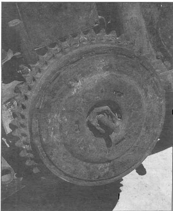
Cobble work to fix — an off-year clutch with the hub nut gouged out by a blunt chisel.
