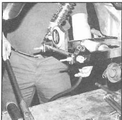
On the 1979 to 1983 models, the swingarm can be widened without being removed from the machine. Do not overheat
