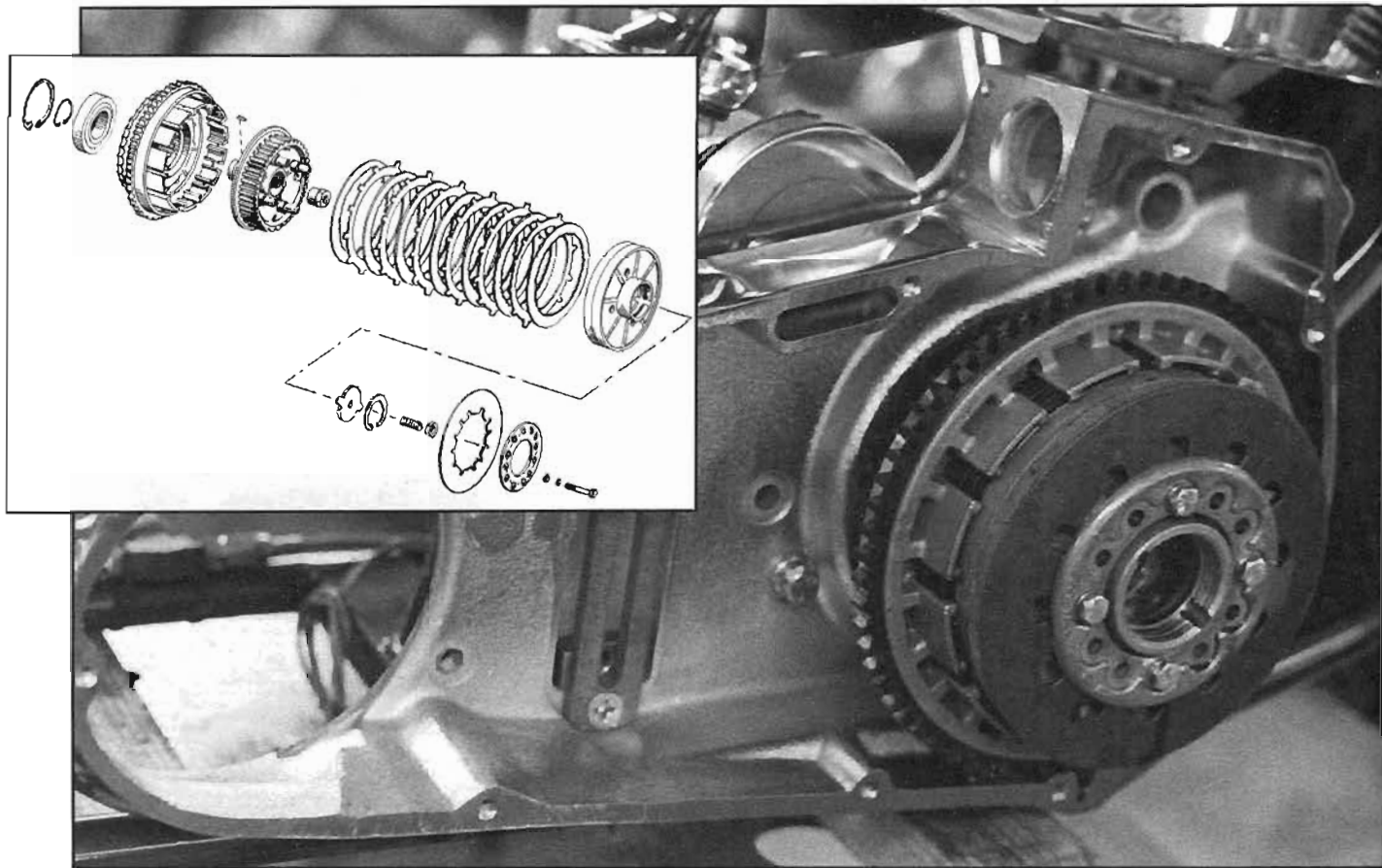
Late-model clutch installed on earlier transmissi
