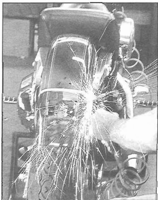
Bob Brovett masked off the fender before firing up a thin wheel on the die grinder and cutting off the bottom half of the fender by hand.
