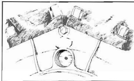
Electric eye plate (left), and 1980 trigger cup. When the leading edge of cutout on cup just breaks electric eye, engine is statically timed.
