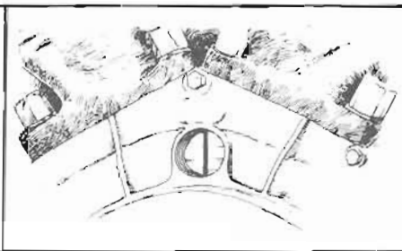
Electric eye plate (left), and 1980 trigger cup. When the leading edge of cutout on cup just breaks electric eye, engine is statically timed.
