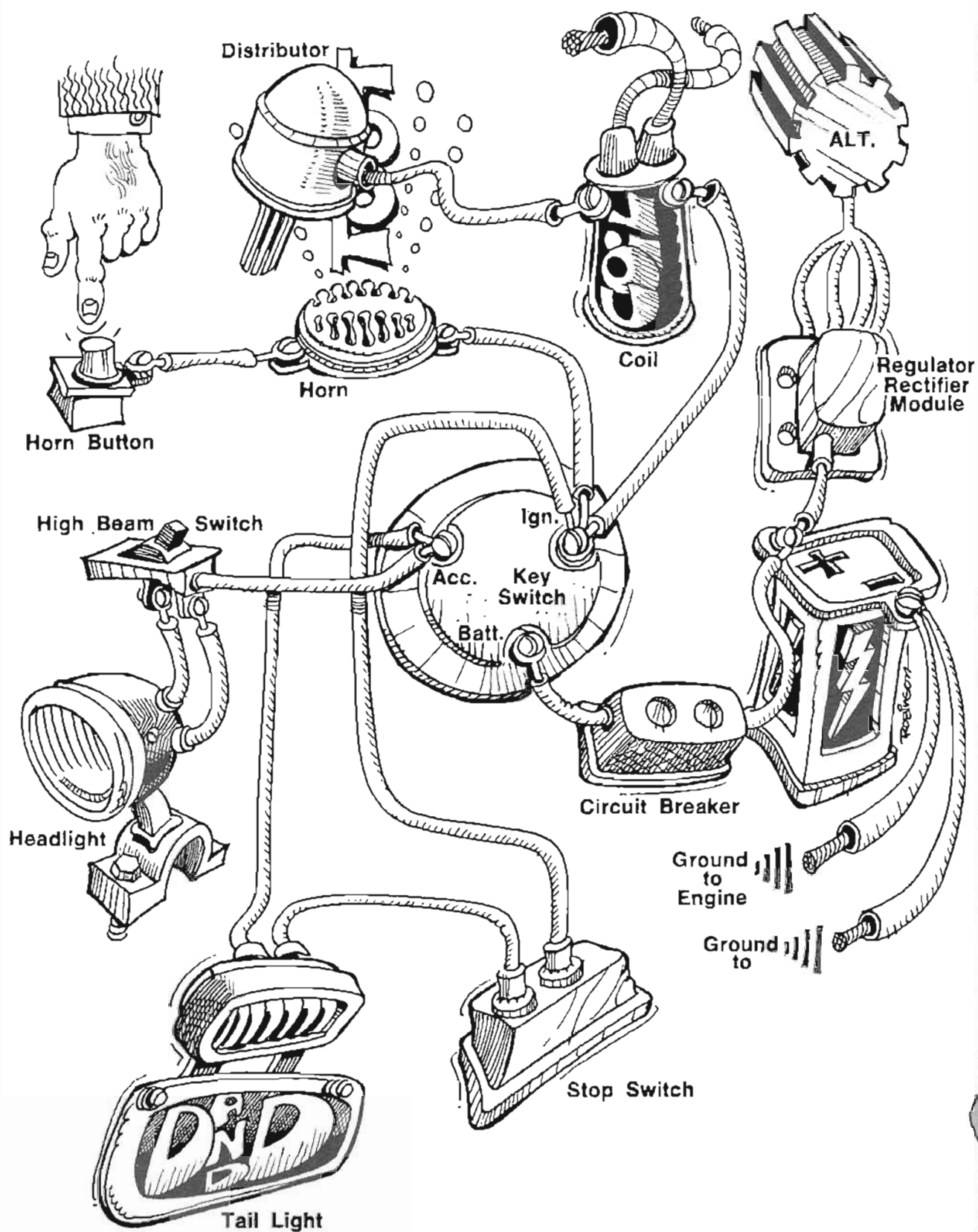
Simplified wiring Diagram for 74s for 70 & Later Alternator
