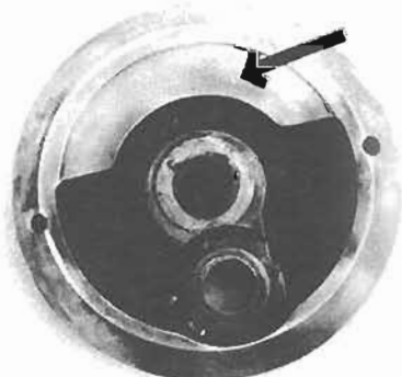
Weight removing must be in balance. Do not machine into this counterbalance.
